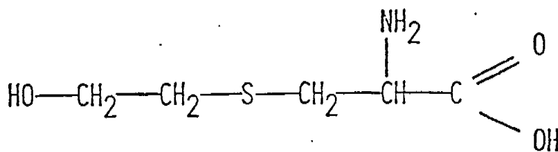
S-(2-HYDROXYETHYL)CYSTEINE
