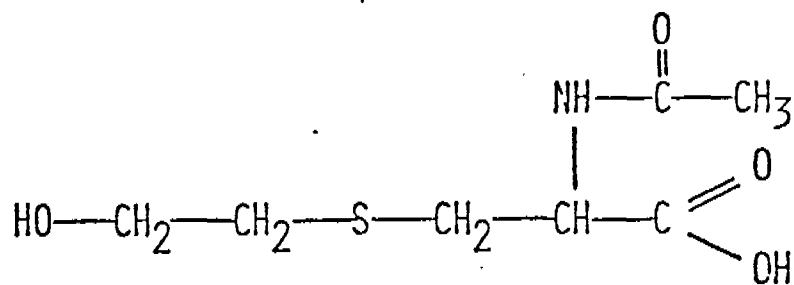
(A) N-ACETYL(S-2-HYDROXYETHYL)CYSTEINE
