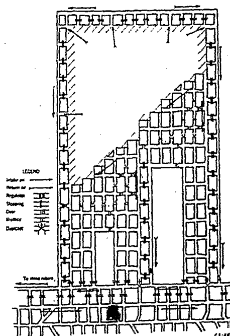
FIGURE 2. Ventilating System Using Bleeders-Pillar Mining.
