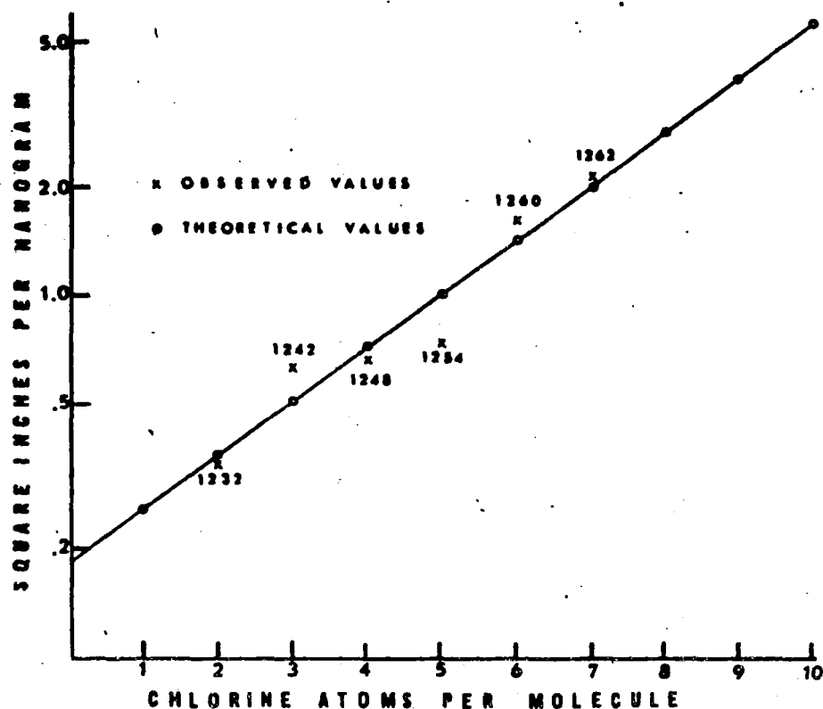
Figure 1. Detector response curve. Response to p,p'-DDE = 2.75 \text{ in}^2/\text{ng} . ( \log y = 0.1512x - 0.7428 )
