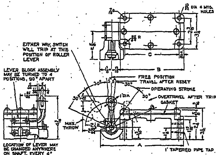
Snap Action Limit Switch with roller lever operator Clockwise and counter-clockwise trip.
