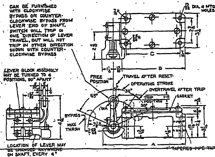
Snap Action Limit Switch with roller lever operator Clockwise and counter-clockwise trip.
