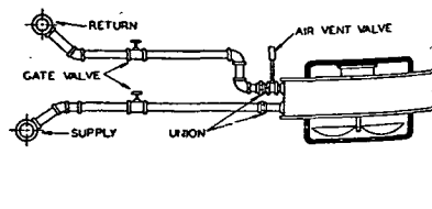
FIG. 9. CONNECTION OF VERTICAL UNIT HEATER TO HOT WATER SYSTEM
