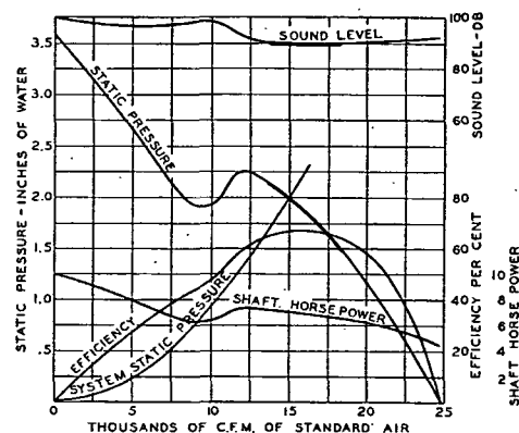
FIG. 2. SOUND LEVEL CHARACTERISTICS OF TYPICAL VANEAXIAL FAN
