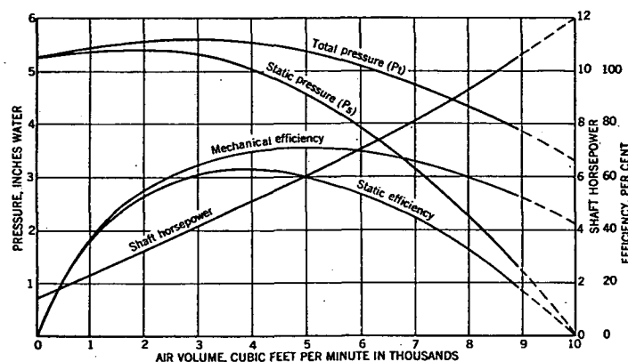
FIG. 1. TYPICAL FAN PERFORMANCE CURVE
