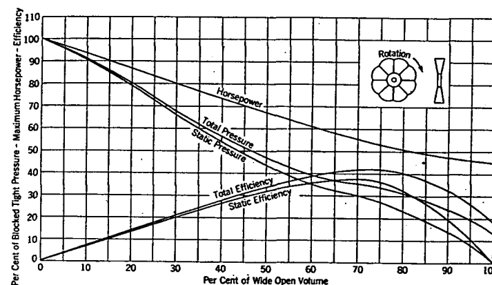
FIG. 2. OPERATING CHARACTERISTICS OF AN AXIAL FLOW FAN WITH BLADES OF UNIFORM THICKNESS
