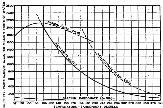
FIG. 3. SOLUBILITY OF CALCIUM SULPHATE AND OF CALCIUM CARBONATE FOR COMPARISON
