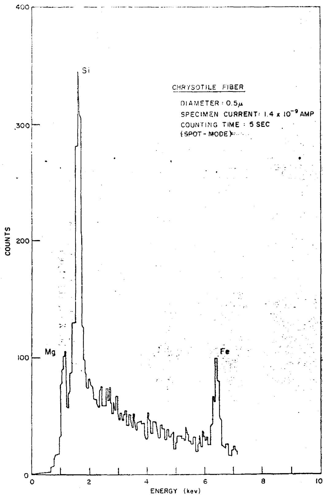
Figure 5. X-ray Spectrum from a 0.5 μ Diameter Chrysotile Fiber
