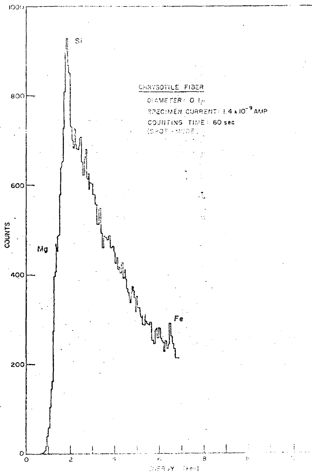
Figure 6. X-ray Spectrum From a 0.1 \mu Diameter Chrysotile Fiber
