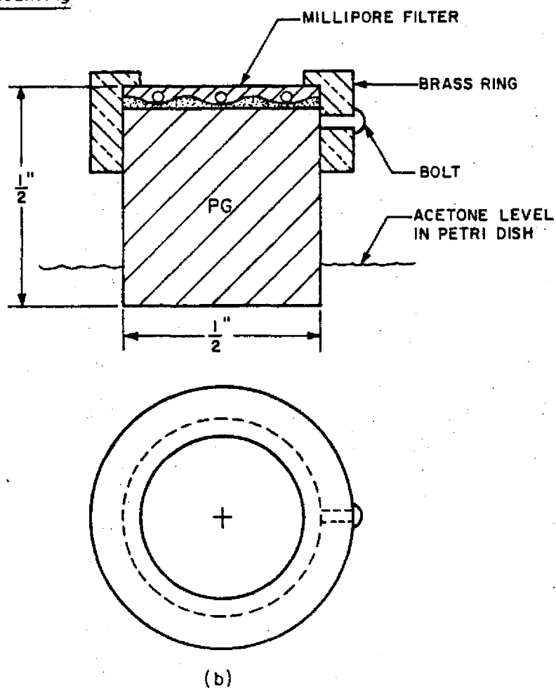
Figure 1. Schematic Diagram of the Steps Involved in Specimen Preparation
