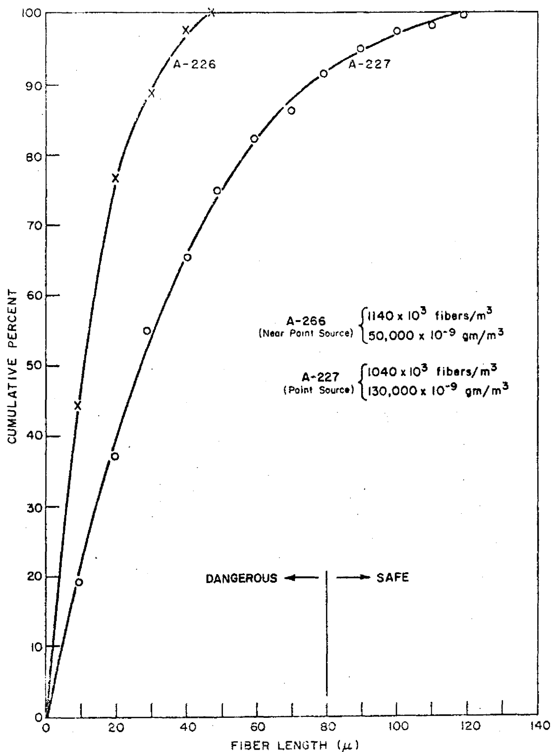
Figure 11. Cumulative Distribution of Fiber Lengths in Point-Source and Near-Point Source Samples
