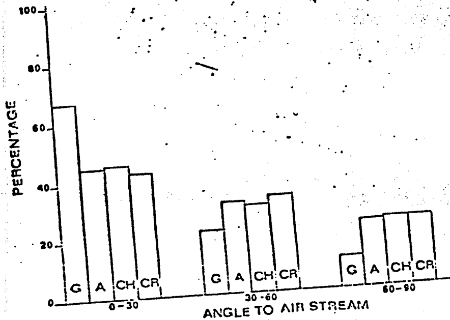
Figure 3: Frequency histograms in which percentage of fibres is plotted against angle to the airstream (axis of duct) in the aerosol spectrometer, for glass, amosite, chrysotile and crocidolite fibres with aspect ratios > 5 .
