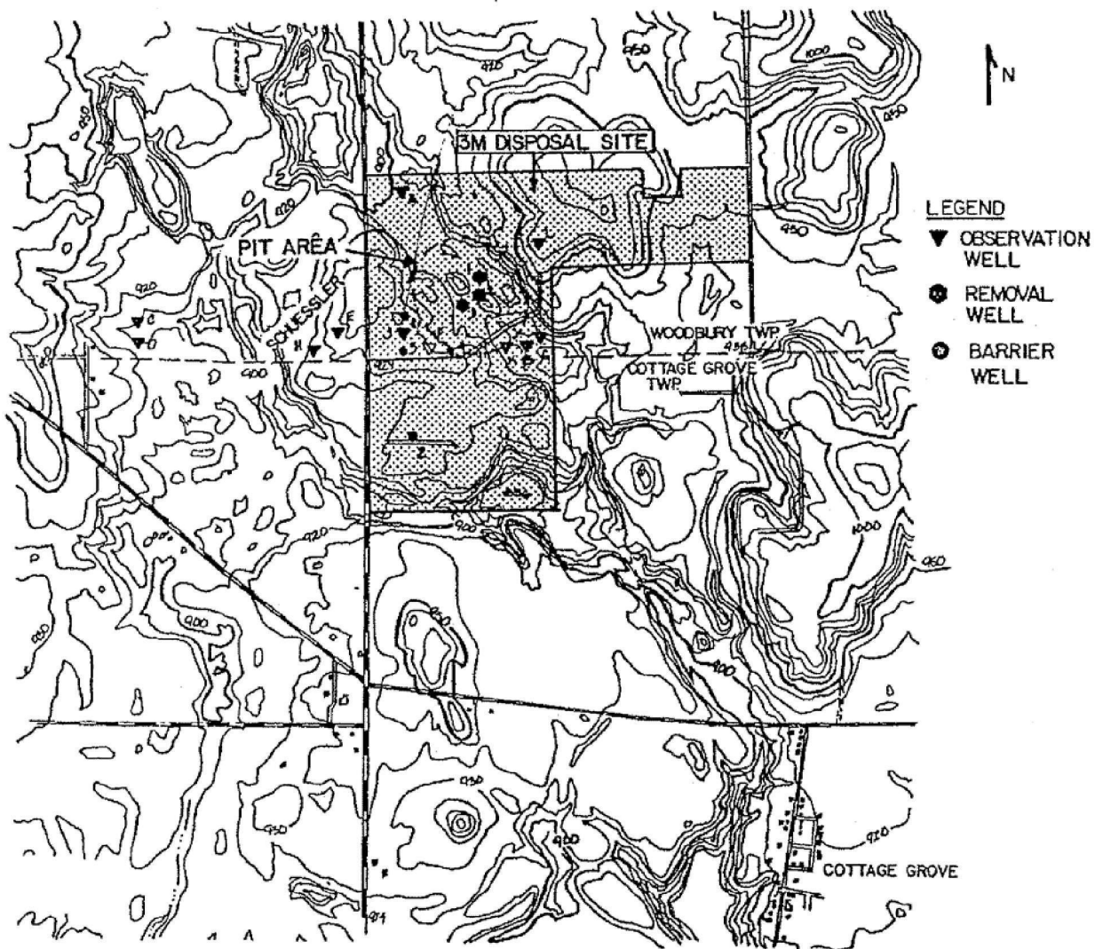
Figure 8-4. Location of contaminated well (Schuessler well) and barrier wells. 1,3
