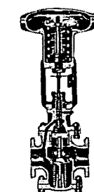
Diaphragm Control Valve Class D-3
