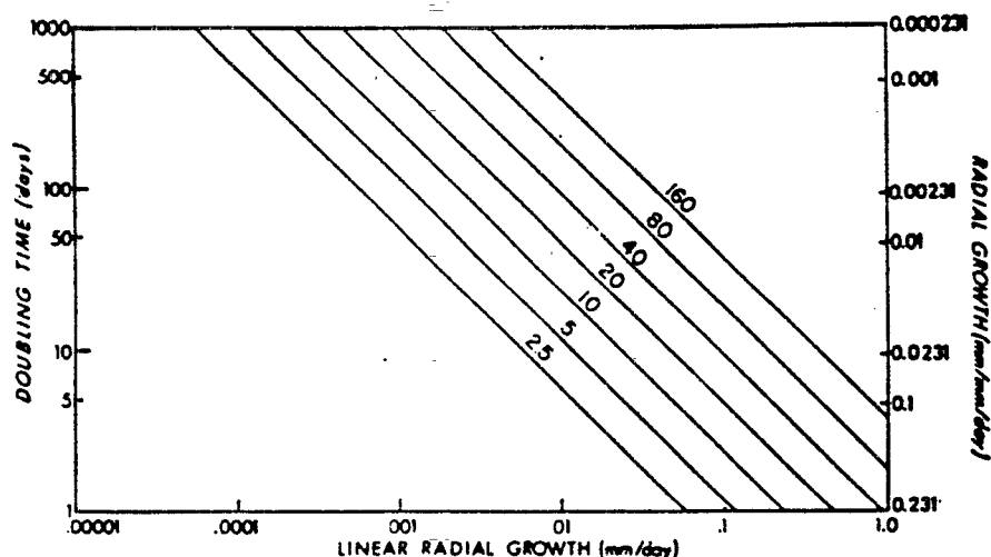
Fig. 3. To use this nomogram, calculate the linear radial growth rate in mm./day as described in the text. Similarly, determine the length of the radius midpoint between the two measurements of tumor size. The slanted lines are the nomograms for the midpoint radii. Project a vertical extension from the calculated growth rate (mm./day) to intersect the line most closely approximating the midpoint radius. From this intersect, extend a line horizontally to obtain an approximation of the doubling time on the left. By extending the horizontal line to the right, one can obtain the exponential radial growth in mm./mm./day.
