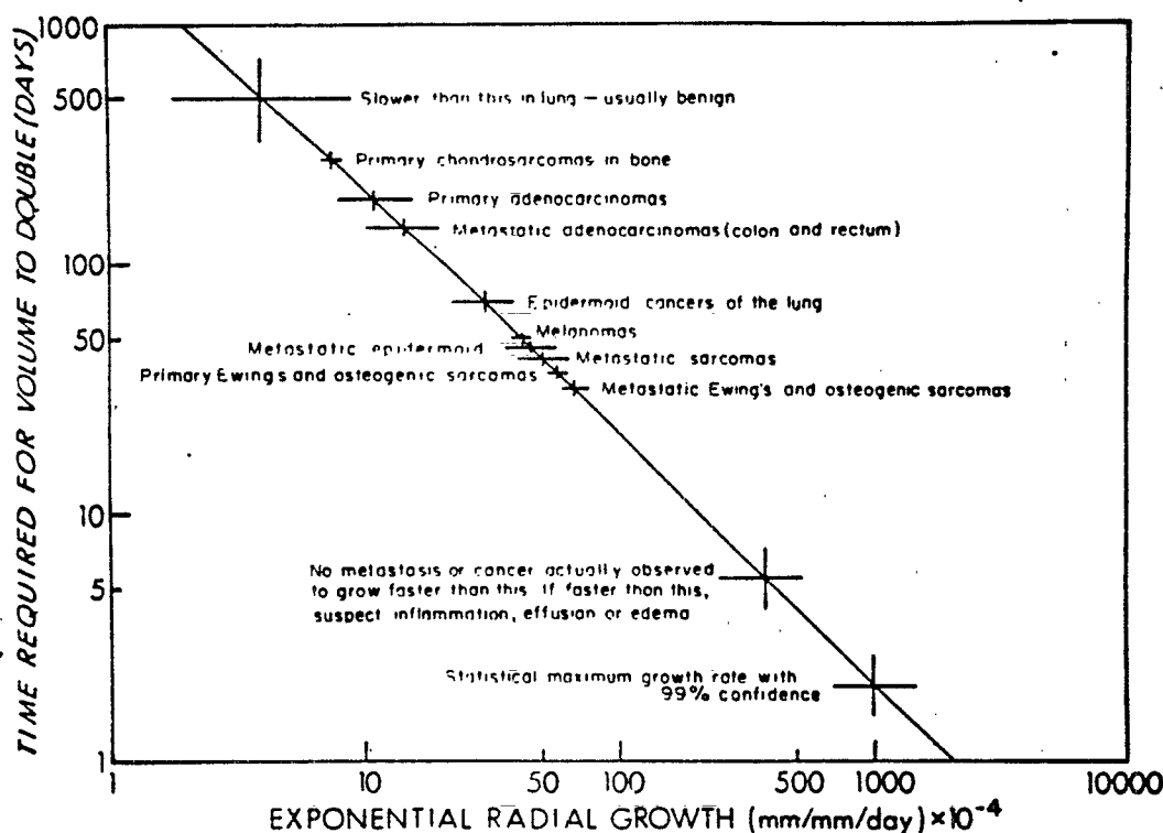
Fig. 4. This nomogram relates the time required in days for a growing spherical cancer to double its volume to the exponential radial growth rate in mm./mm./day. By multiplying the exponential radial rate by 3 and moving the decimal place to the right three places, still an additional parameter is obtained—the net gain in cancer cells per thousand existing cancer cells per day.
