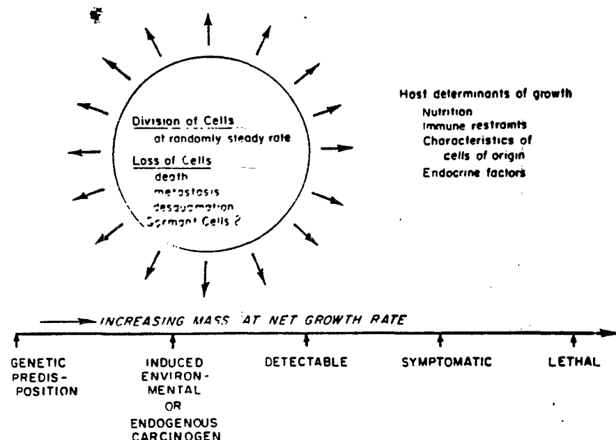
Fig. 1. Kinetic model of an untreated cancer. A solid cancer growing in the lung is a dynamic mass of tissue on which many factors are acting simultaneously. These variable factors produce a net effect on growth which produces grossly measurable growth rates characterizing various cancers (and pulmonary metastases) and affecting longevity.
