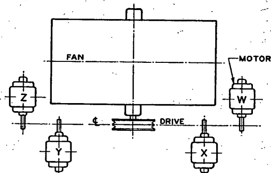
FIG. 8. MOTOR POSITION, BELT OR CHAIN DRIVE
