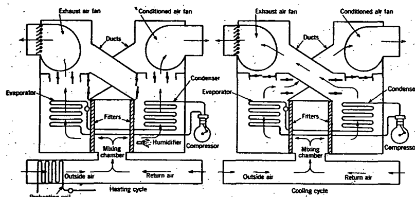
FIG. 8. SCHEMATIC OPERATION OF REVERSED CYCLE CONDITIONING SYSTEM
