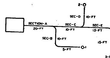
FIG. 11. DUCT LAYOUT FOR EXAMPLE 5
