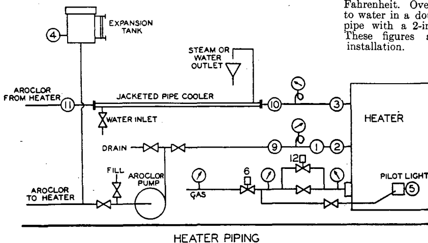
Figure 2. Cooler, Pump, and Expansion Tank
