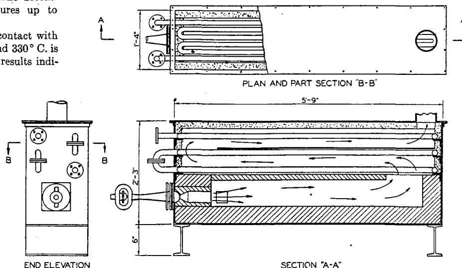
Figure 1. Heater
