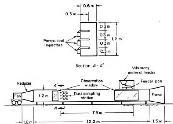
Figure 2. Dust entrainment tunnel schematic
