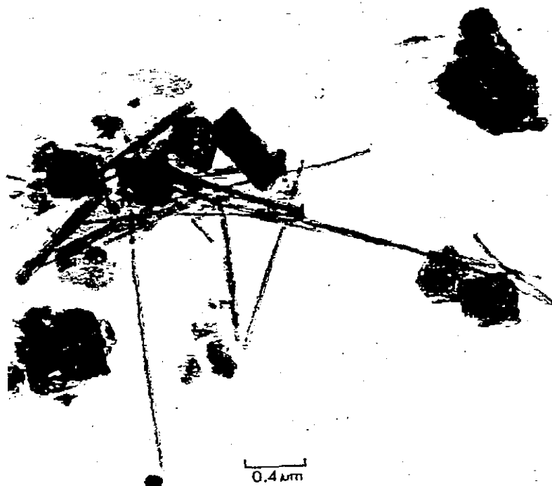
Figure 2 — Electron photomicrograph of air sample taken during sanding of taping compound. Numerous chrysotile fibers are visible, most of which are shorter than 1 micrometer. They would not be visible by optical microscopy. Granular particles are micas, clays and plaster of Paris.
