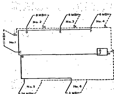
FIG. 13. TWO-PIPE REVERSED RETURN GRAVITY SYSTEM (EXAMPLE 5)
