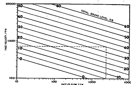
FIG. 9. AIR FLOW AND SOUND LEVEL CHART.
