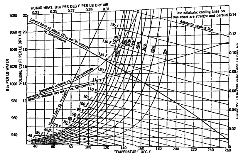
FIG. 6. PSYCHROMETRIC CHART
