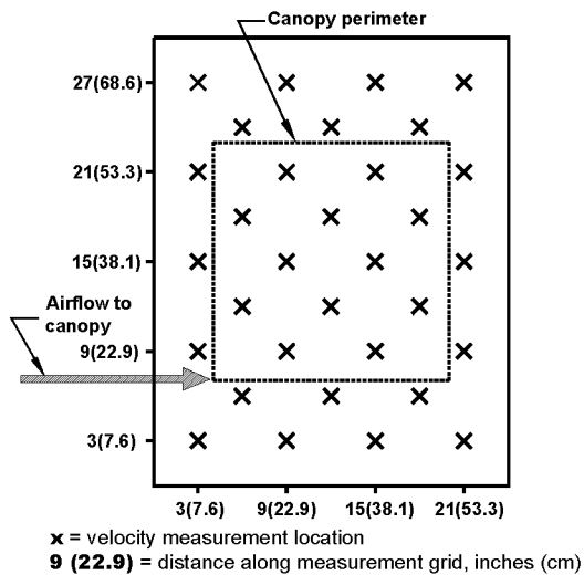
Figure 2. Velocity measurement grid
