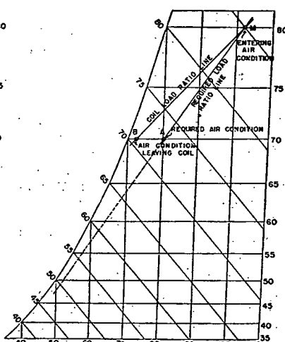
FIG. 3. PSYCHROMETRIC LAYOUT FOR COIL SELECTION USING REHEAT
