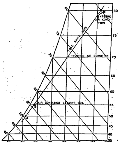
FIG. 2. PSYCHROMETRIC LAYOUT FOR COIL SELECTION
