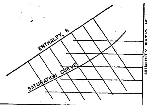
FIG. 3. BASIC COORDINATES OF A.S.H.V.E. PSYCHROMETRIC CHART
