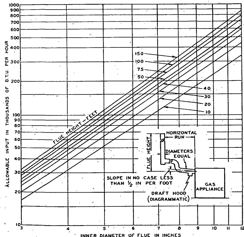
FIG. 6. ALLOWABLE BTU INPUT TO CIRCULAR FLUES FOR DOMESTIC GAS APPLIANCES WITH DRAFT HOODS
