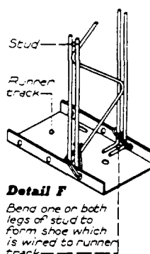
Short Studs Over Opening
