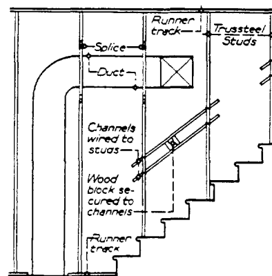
Handrail Grounds and Ventilating Duct
