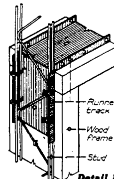
Detail E NOTE—This detail applies also to wood door bucks for wood trim.
