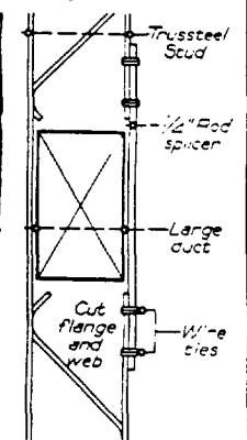
Detail of Duct
