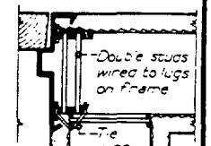
SCALE 1 1/2" = 1' 0" Alternate Jamb
