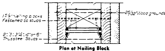
Plan at Nailing Block
