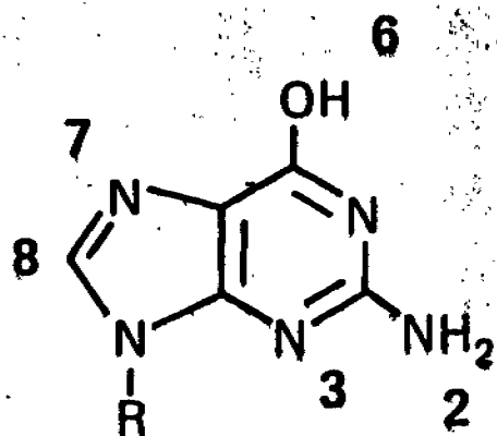
Guanine
