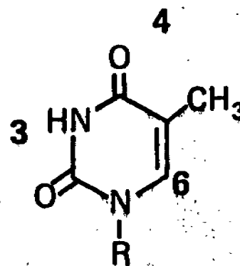
Thymine
