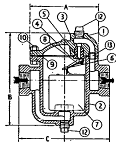
Cross-section of No. 800, 811, 812 and 813 traps for standard angle pipe through pipe connections.
