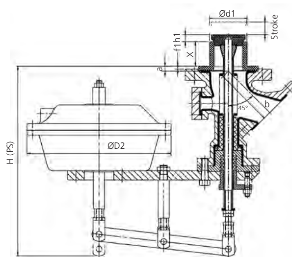
Flat seat with standard actuator* Standard seat with side-mounted actuator
