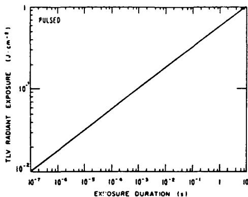
Figure 7a — TLV for laser exposure of skin and eyes for far-infrared radiation (wave-lengths greater than 1.4 \mu\text{m} ).
