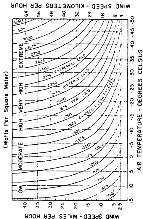
Figure 2 — Wind chill cooling rates. Adapted from Canadian Department of the Environment, Atmospheric Environment Service.
