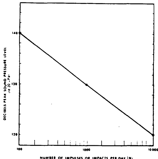
Figure 9—Threshold Limit Values for Impulse/Impact Noise.
