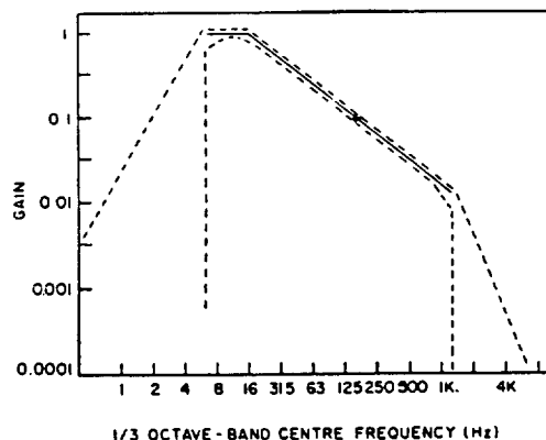
Figure 4—Gain characteristics of the filter network used to frequency-weight acceleration components (continuous line). The filter tolerances (dashed lines) are provisional, and are those contained in ISO 5349.
