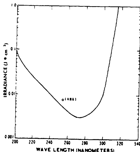
Figure 11 — Threshold Limit Values for Ultraviolet Radiation.
