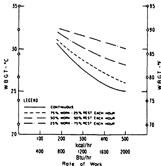
Figure 1—Permissible Heat Exposure Threshold Limit Values.
