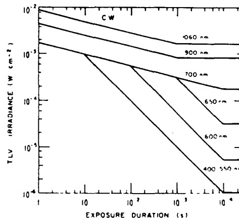
Figure 6b — TLV for intrabeam (direct) viewing of CW laser beam (400-1400 nm).
