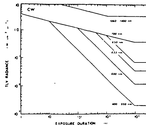
Figure 8b — TLV for extended sources or diffuse reflections of laser radiation (400-1400 nm).
