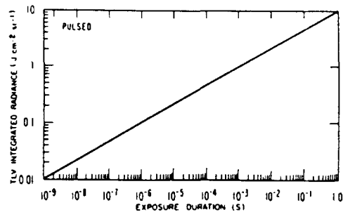
Figure 8a — TLV for extended sources or diffuse reflections of laser radiation (400-700 nm).
