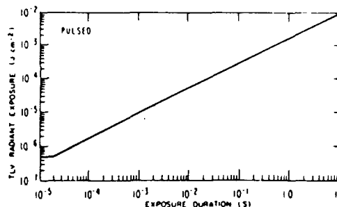
Figure 6a — TLV for intrabeam (direct) viewing of laser beam (400-700 nm).
