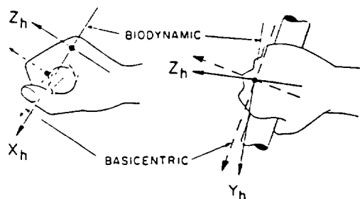
Figure 3—Biodynamic and basicentric coordinate systems for the hand, showing the directions of the acceleration components (ISO 5349).
