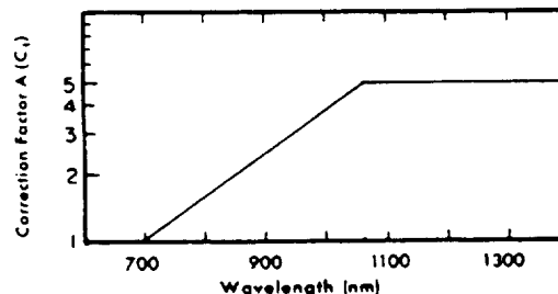
Figure 5—TLV correction factor for \lambda = 700 -1400 nm.* (* For \lambda = 700 -1049 nm, C_A = 10^{(0.0024(\lambda - 700))} ; For \lambda = 1050 -1400 nm, C_A = 5 .)
