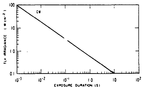
Figure 7b — TLV for CW laser exposure of skin and eyes for far-infrared radiation (wave-lengths greater than 1.4 \mu\text{m} ).
