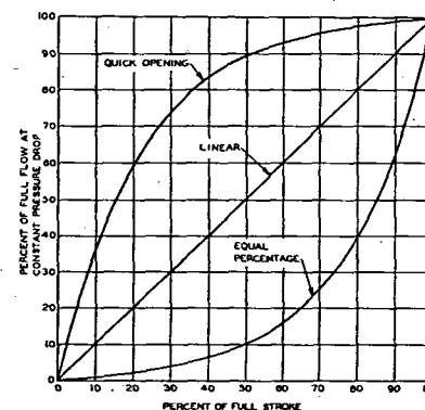
Fig. 6.... Typical Flow Characteristics
