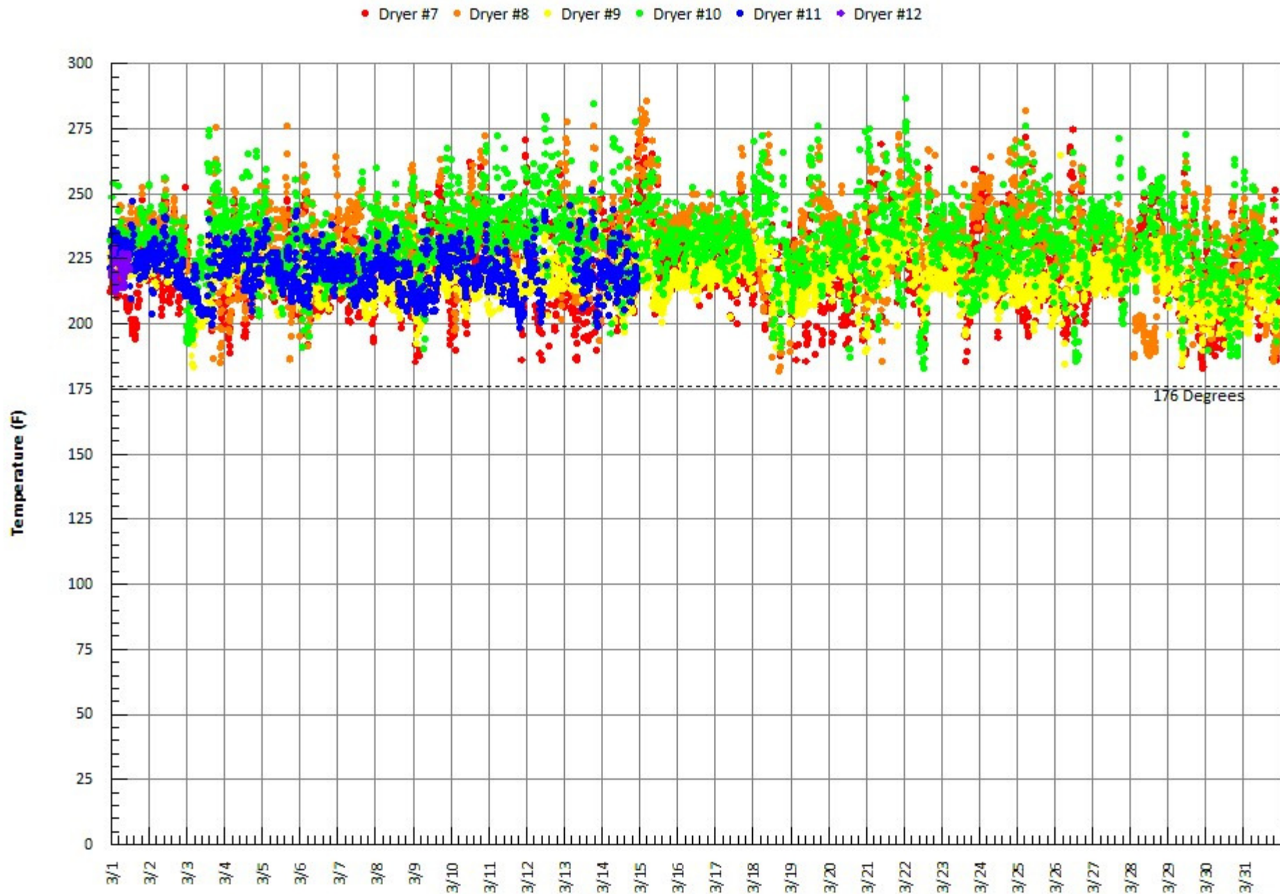
Graph #2 - Dryer Discharge Temperature - North Dryers - March 2021
