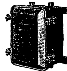
CR7006-D51FS quiet magnetic switch. For full-voltage starting of squirrel-cage motors up to 5 hp, 220 volts. For applications where quiet operation is required, such as on fans or domestic air-conditioning systems
