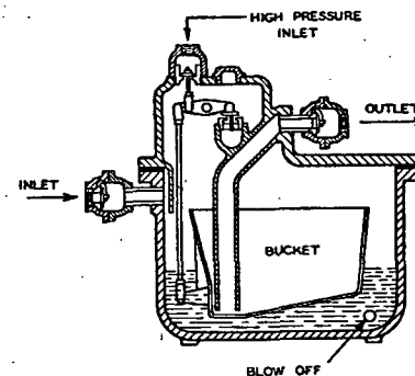
FIG. 32. LIFTING TRAP
