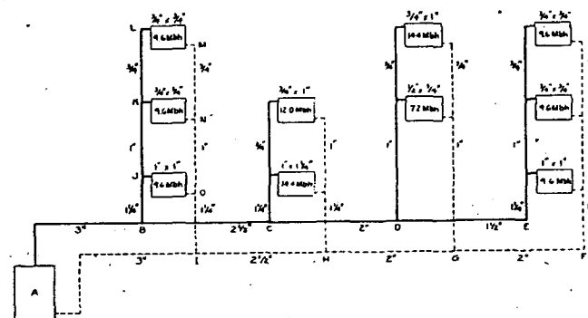
FIG. 7. A TWO-PIPE DIRECT RETURN GRAVITY CIRCULATION SYSTEM
