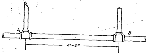
FIG. 9. RADIATOR CONNECTIONS FOR A ONE-PIPE SYSTEM ILLUSTRATING THE INFLUENCE OF THE PRESSURE DROP IN THE MAIN UPON THE CIRCULATION THROUGH THE RADIATOR
