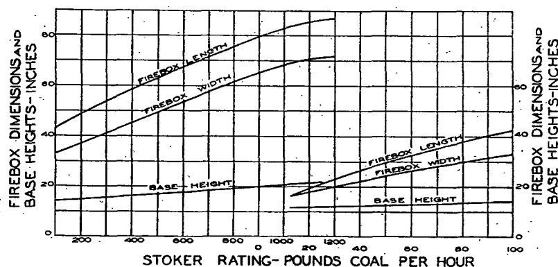
FIG. 11. SUGGESTED MINIMUM FIREBOX DIMENSIONS AND BASE HEIGHTS 4
