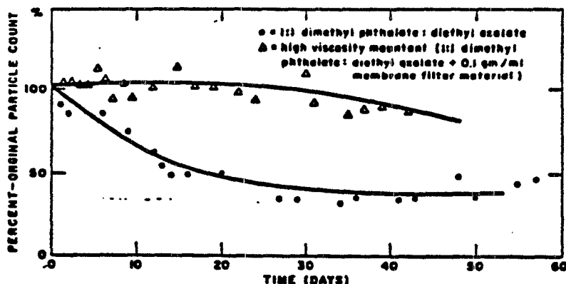
FIG. 2. Decrease in percentage of original particle count with time for the original 1:1 dimethyl phthalate-diethyl oxalate mixture and for the high viscosity mixture containing 0.1 g/ml of membrane filter material.
