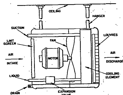
FIG. 12. SUSPENDED PROPELLER FAN TYPE COOLING AIR CONDITIONING UNIT
