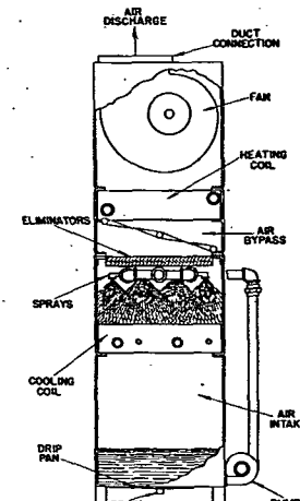
FIG. 15. SPRAY TYPE AIR CONDITIONING UNIT
