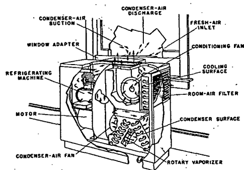
FIG. 13. PORTABLE SELF-CONTAINED CONDITIONING UNIT FOR COOLING
