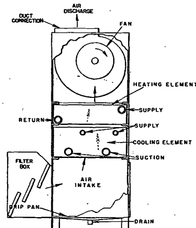
FIG. 14. VERTICAL REMOTE TYPE ALL-YEAR-ROUND CONDITIONING UNIT
