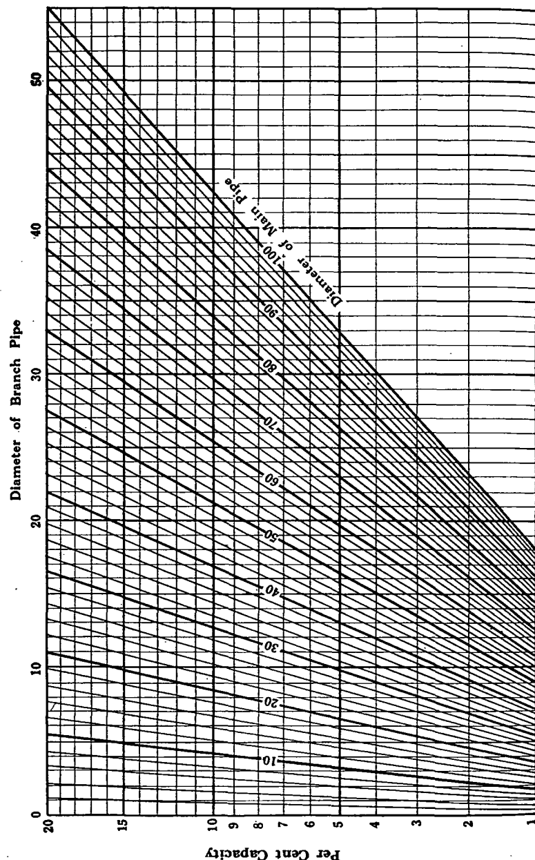
FIG. 4. MAIN AND BRANCH PIPES FOR EQUAL FRICTION PER FOOT OF LENGTH (1 TO 20 PER CENT CAPACITY)
