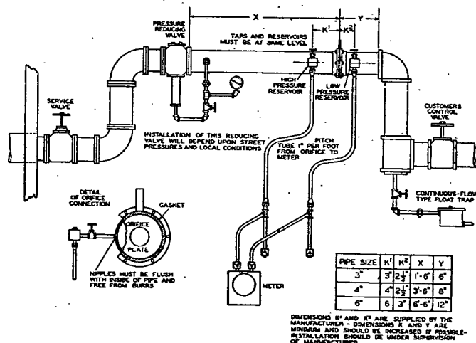
FIG. 7. ORIFICE METER STEAM SUPPLY CONNECTION
