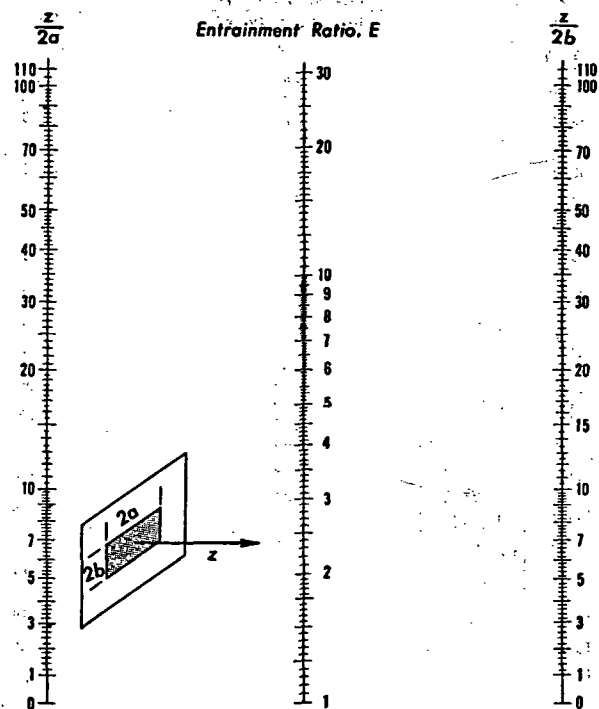
FIG. 11. NOMOGRAM FOR ENTRAINMENT RATIOS OF ROUNDED, RECTANGULAR JET SOURCES
