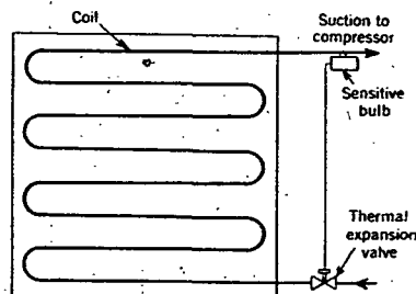
FIG. 8. DIRECT-EXPANSION COIL WITH THERMAL VALVE SYSTEM
