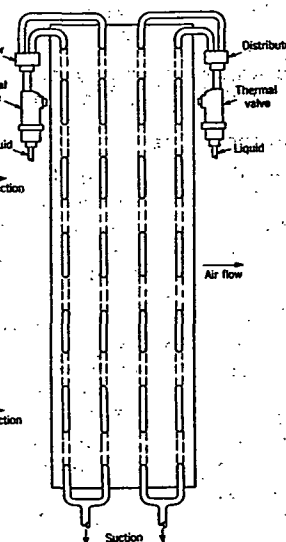
FIG. 11. ARRANGEMENT FOR DEPTH CONTROL
