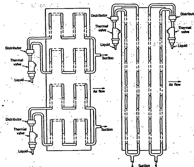
FIG. 10. ARRANGEMENT FOR FACE CONTROL
