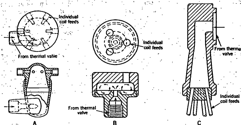
FIG. 9. TYPES OF REFRIGERANT FEED DISTRIBUTING HEADS
