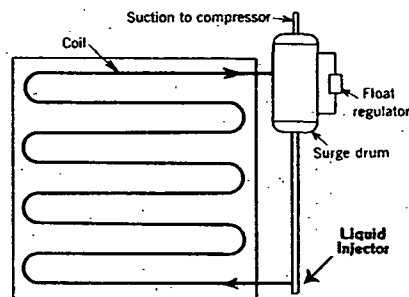
FIG. 7. DIRECT-EXPANSION COIL WITH FLOODED SYSTEM
