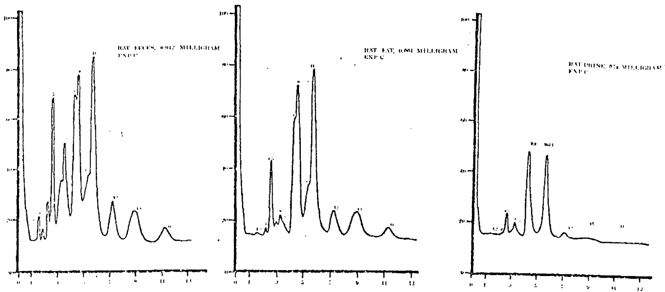
FIG. 4. Gas chromatogram for rat feces, fat and urine (a plot of detector response vs time).
