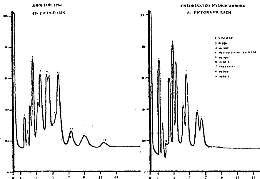
FIG. 1. Gas chromatograms for Aroclor 1254 and chlorinated hydrocarbon standards. (A plot of detector response vs time.)
