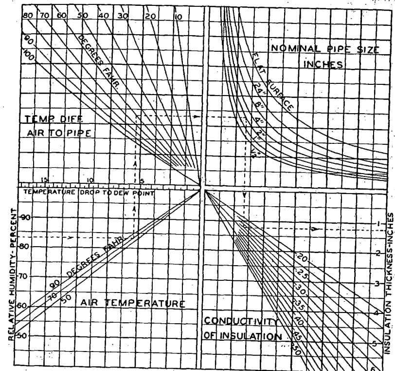
FIG. 5. THICKNESS OF PIPE INSULATION TO PREVENT SWEATING*
