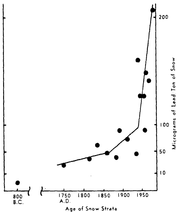
FIGURE 1. The amount of industrial lead in the snow was measured in samples taken from the Greenland Ice Sheet. The more recent the sample, the higher the concentration of lead.
