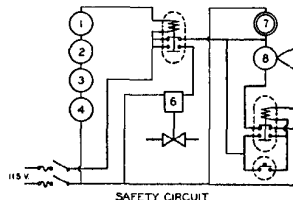
Figure 3. Control and Safety Circuit
