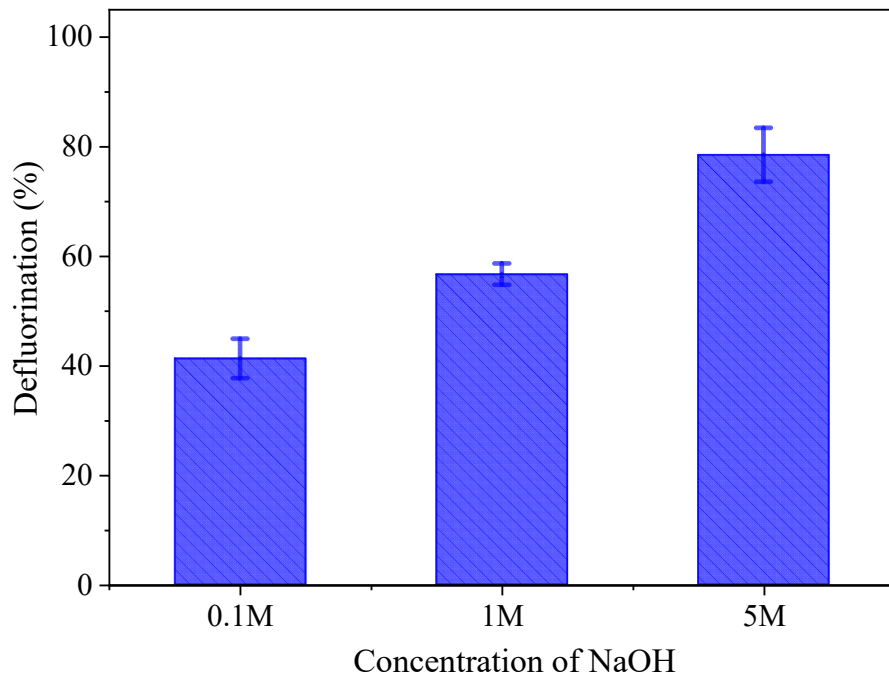
Figure 4.3.3 Defluorination observed during alkaline hydrothermal treatment of AFFF #1 solution with (a) different reaction temperatures, and (b) different concentrations of NaOH amendment. Reaction conditions: AFFF diluted 1-to-1000, 5 M NaOH reaction for 90 min in panel (a), AFFF diluted 1-to-1000, 0.1-5 M NaOH reaction for 15 min under 350°C in panel (b).
