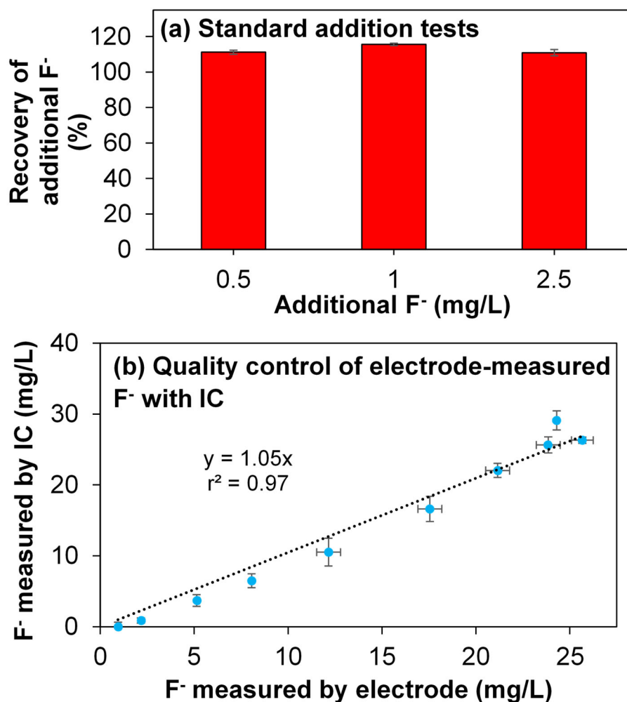
Figure 3.5.1 Accuracy evaluation of electrode measurement of fluoride ion concentration. (a) Electrode measured recovery rates of additional fluoride ions added to the reacted samples (50 mg·L -1 PFOS, 1 mol·L -1 NaOH; 350 °C, 90 min). (b) Comparison of IC- and ISE-measured fluoride ion concentrations of reacted PFOS samples for different reaction time periods. Each symbol represents one sample collected at a certain reaction time. The higher yield of fluoride ion was due to the longer reaction time. Reaction conditions: PFOS (50 mg/L), NaOH (1 mol/L), 350 °C, 0-480 min. Error bars represent min/max values observed for duplicate experiments (smaller than symbol if not visible).
