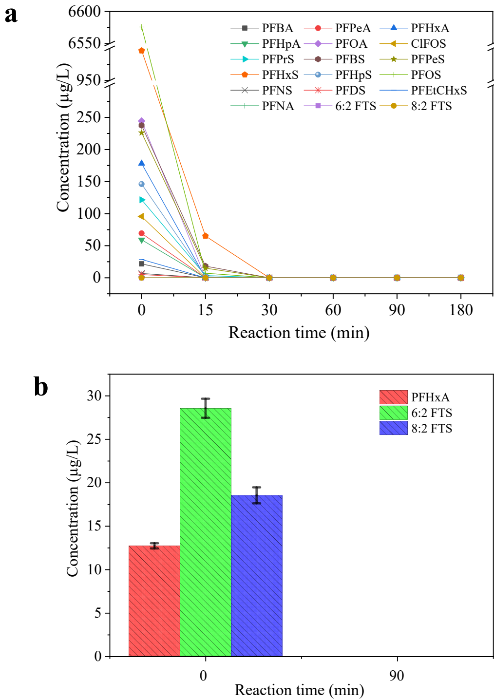
Figure 4.3.4 Removal of targeted PFASs observed following alkaline hydrothermal treatment of (a) AFFF #1 solution, and (b) AFFF #2 solution.
