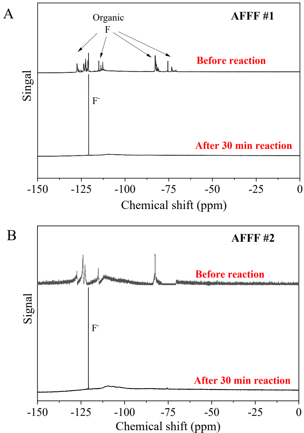
Figure 4.3.7 ^{19}\text{F} -NMR spectra of (a) diluted AFFF #1 (diluted 1-to-2) and (b) diluted AFFF #2 (diluted 1-to-4) before and after hydrothermal reaction for 30 min. Reaction conditions: 5 M NaOH amendment, 350°C.
