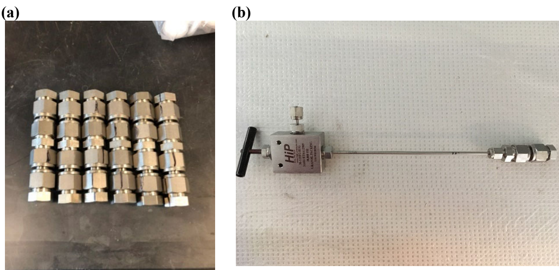
Figure 3.4.1 (a) Mini-tube batch reactors used for hydrothermal treatment experiments. (b) Reactors outfitted with specialized gas sampling valve.
