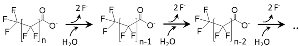
Figure 4.6.2 Proposed mechanism for decomposition of PFOA under hydrothermal conditions.
