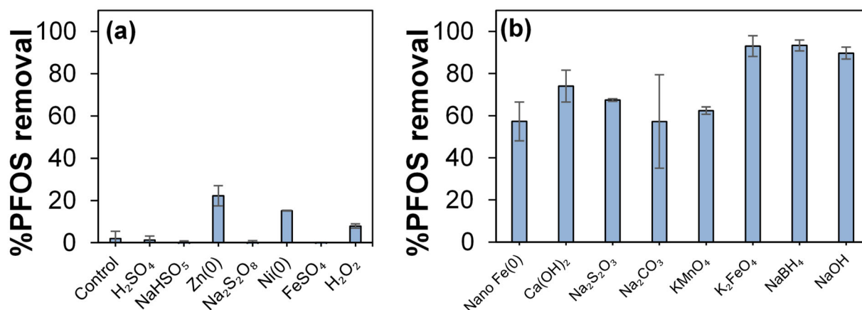
Figure 4.1.2 PFOS removal measured in reaction solutions amended with (a) seven reagents that yielded the lowest extent of defluorination, (b) eight reagents that yielded the greatest degree of defluorination (as shown in Figure 4.1.1). Error bars represent min/max values observed for duplicate experiments.
