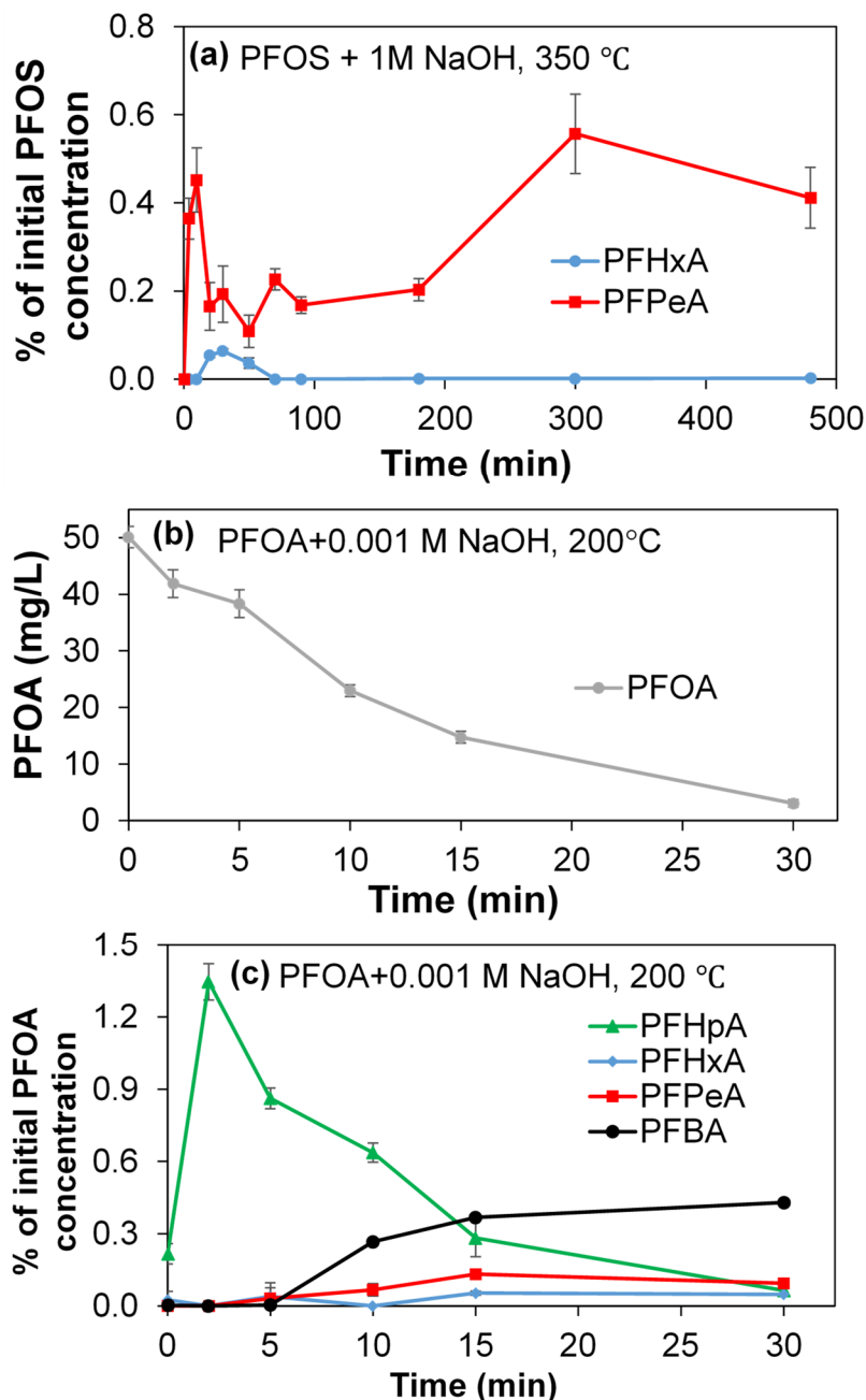
Figure 4.2.3 Intermediate products observed during hydrothermal treatment of (a) 50 mg/L PFOS with 1 M NaOH at 350 °C, (b, c) 50 mg/L PFOA with 0.001 M NaOH at 200 °C. Error bars represent min/max values observed for duplicate experiments (smaller than symbol if not visible).
