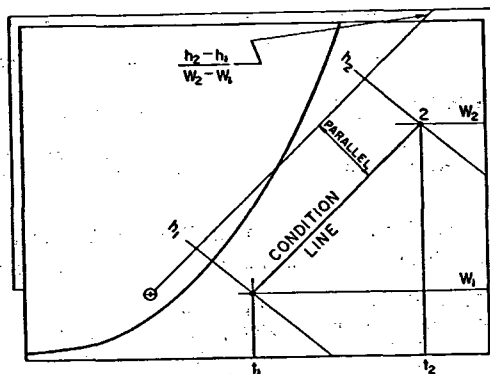
FIG. 16. SOLUTION OF EXAMPLE 8 ON A.S.H.V.E. PSYCHROMETRIC CHART
